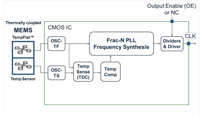
Figure 32. Block Diagram – TC-MO
