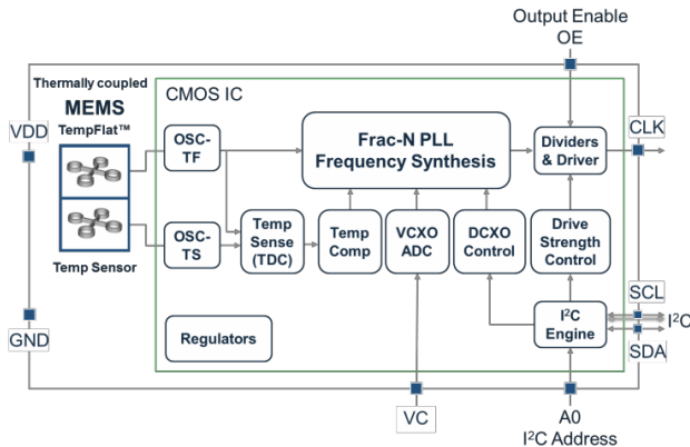
Figure 318. Elite Architecture
