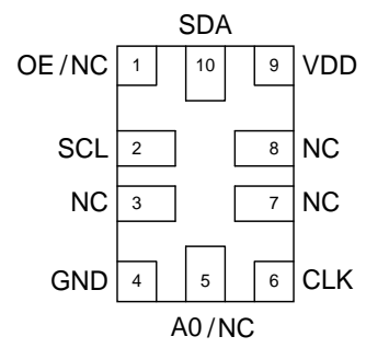
Figure 5. DCTC-MO
