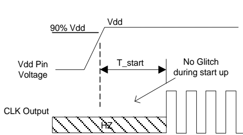
Figure 11. Startup Timing
