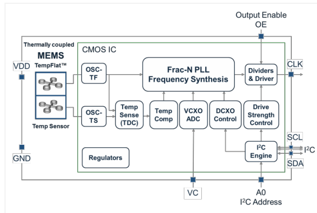
Figure 1. MO5357 Block Diagram
