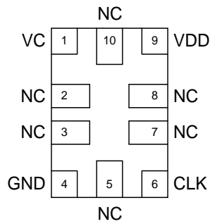
Figure 4. VCTC-MO
