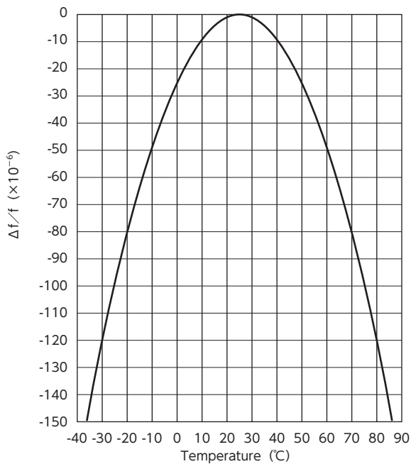
Temperature Characteristics for BT Cuts
