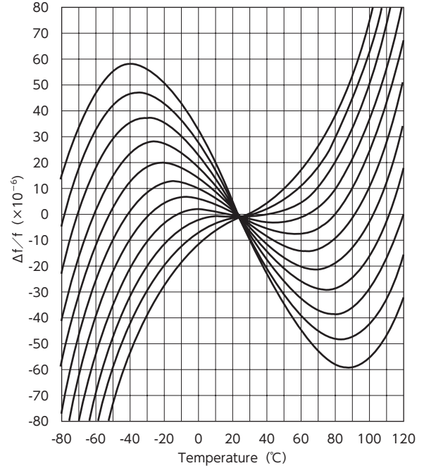
Temperature Characteristics for AT Cuts
