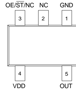
Figure 1. Pin Assignments
